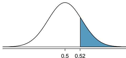
Figure 6.1: Sampling distribution of the sample proportion if the null hypothesis is true for Example 6.5. The p-value for the test is shaded.
