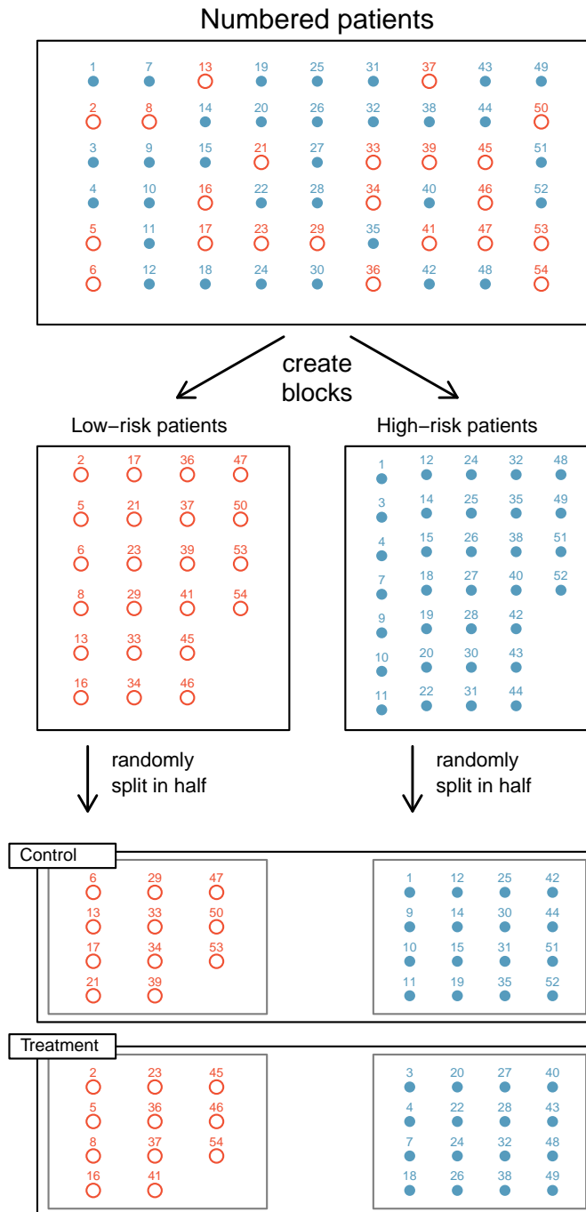
Figure 1.15: Blocking using a variable depicting patient risk. Patients are first divided into low-risk and high-risk blocks, then each block is evenly separated into the treatment groups using randomization. This strategy ensures an equal representation of patients in each treatment group from both the low-risk and high-risk categories.
