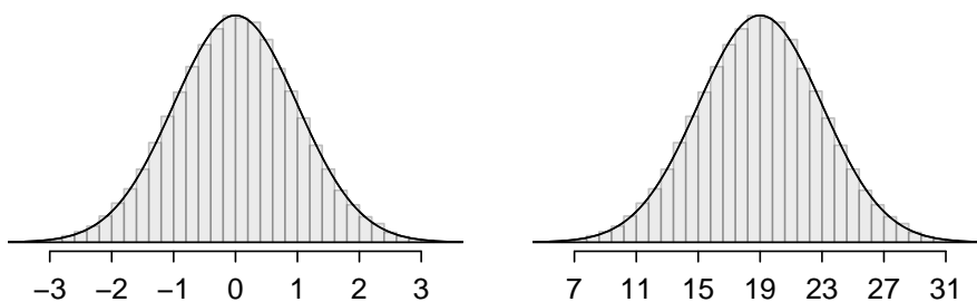
Figure 3.2: Both curves represent the normal distribution, however, they differ in their center and spread. The normal distribution with mean 0 and standard deviation 1 is called the standard normal distribution .
